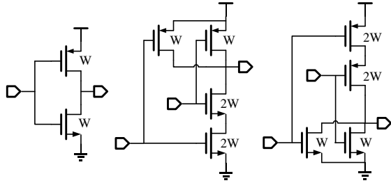
Figure 2. Logical efforts of INVX1, NAND2X1 and NOR2X1 gates that the stack PMOS and
