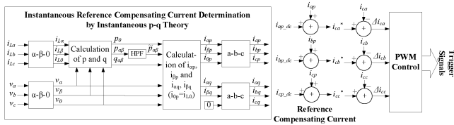
Figure 7. Control block diagram for the three-phase four-wire LC-HAPF
