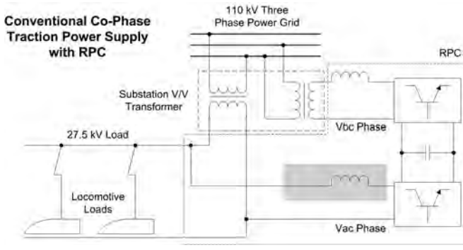
Fig. 1. Circuit configuration of the conventional cophase traction power supply system with RPC.
