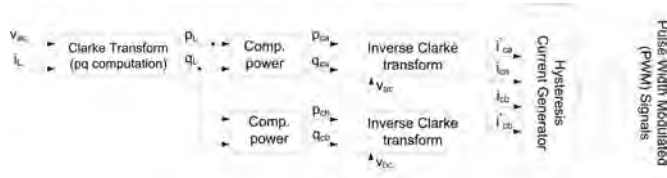
Fig. 11. Control block diagram of the HPQC for cophase traction power supply compensation.
