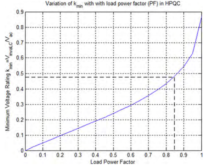
Fig. 10. Curve showing the variation of HPQC minimum voltage rating ( k_{min} ) with load PF.
