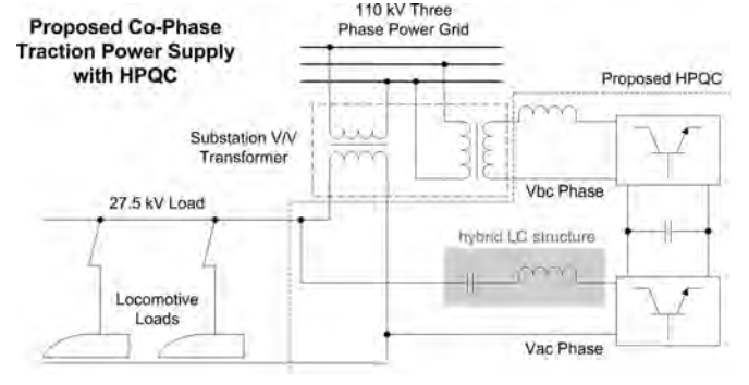
Fig. 2. Circuit configuration of the proposed cophase traction power supply with HPQC.
