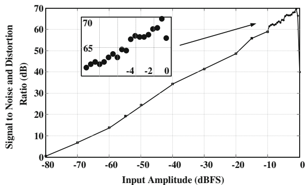
Fig. 19 SNDR versus input signal amplitude
