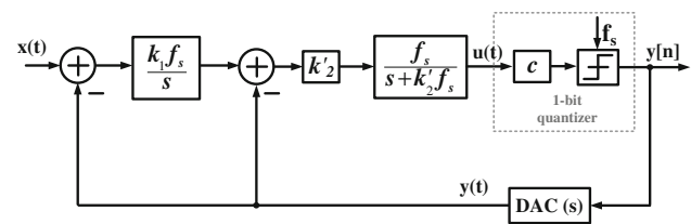
Fig. 6 Analytical model for the loop function optimization of the AP CT \Delta\Sigma modulator
