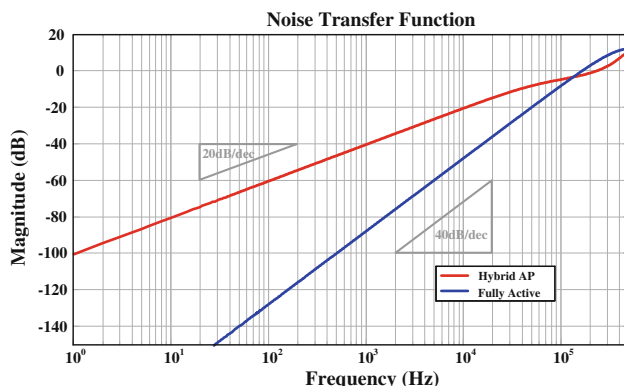
Fig. 5 Calculated NTF for the un-optimized hybrid AP and the active CT \Delta\Sigma modulator
