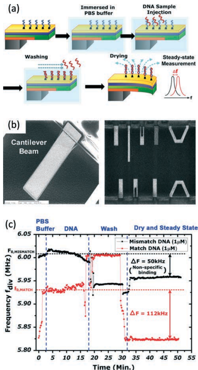
Fig. 6 A CMOS cantilever-based biosensor for DNA detection. (a) The operation procedures of the biosensor. After post-processing to implement the cantilever on the CMOS chip, the captured DNA is immobilized on the Au surface of the cantilever. Then, the cantilever is immersed in the PBS buffer and the sample of interest is injected around the cantilever to allow hybridization of DNA. After washing off the unbound biomolecules, the cantilever is left to dry. After all of the water molecules are evaporated, the matched target DNA will stay on the Au surface. Their masses incur bending of the cantilever and an embedded piezoresistor implemented by N+ polysilicon is entailed to sense this bending, and transduce it to variation of its own resistance, causing a frequency shift on the ring-type oscillator. (b) An SEM image showing the cantilevers. In order to allow the cantilever to bend freely in air, the surrounding materials, such as the insulating dielectrics and p-substrate underneath, have to be etched away, creating a suspended cantilever. (c) Experimental results for the biosensor. The resistance variation of the polysilicon piezoresistor, attributed to the bending of the cantilever, incurs a deviation of the oscillating frequency. After DNA sample injection, and washing and drying steps, the final steady-state frequency can be measured to selectively quantify the concentration of the target DNA inside the sample, with a limit-of-detection of 1 pM, from the hepatitis B virus. Reproduced with permission from ref. 46. Copyright 2013 IEEE.
