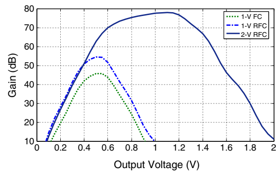
Figure 13. Open-loop gain versus output voltage. The common-mode voltages are V_{cm,1-V FC} = 0.5 V, V_{cm,1-V RFC} = 0.5 V and V_{cm,2-V RFC} = 1 V.
