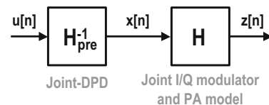
Fig. 3 Proposed joint-DPD for calibration of I/Q imbalance and PA nonlinearity together
