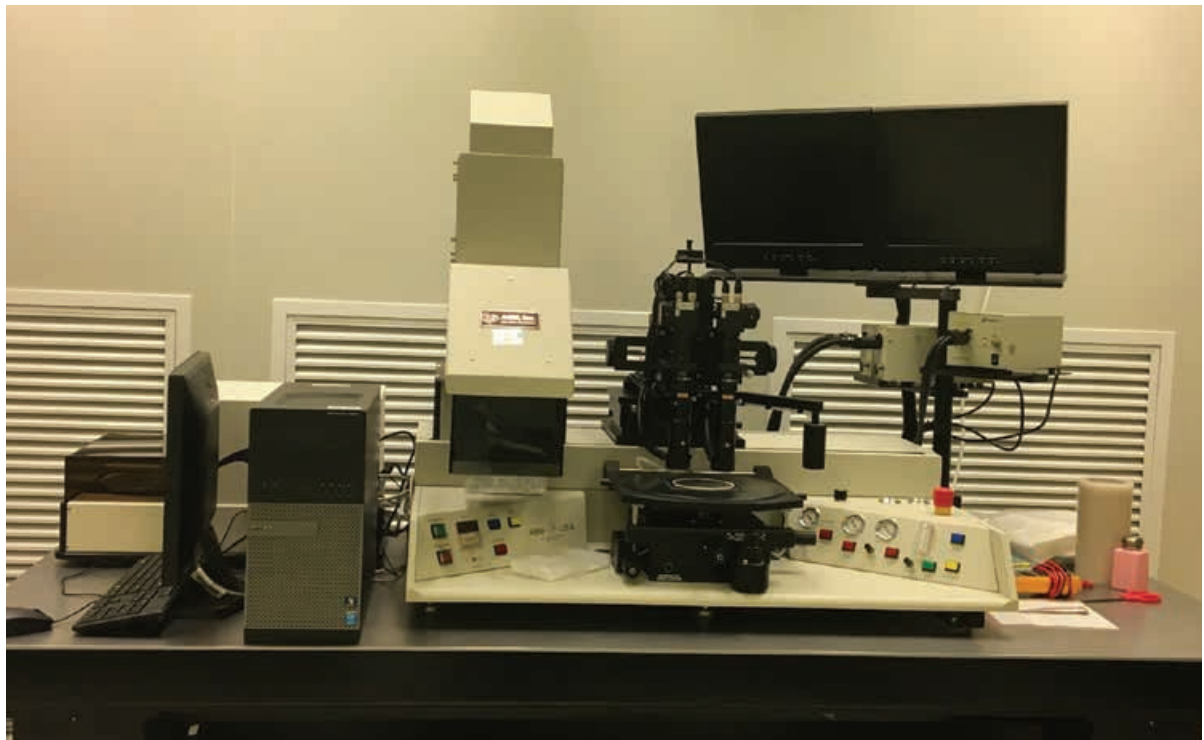
ABM Manual High Resolution Mask Aligner and UV Exposure System
